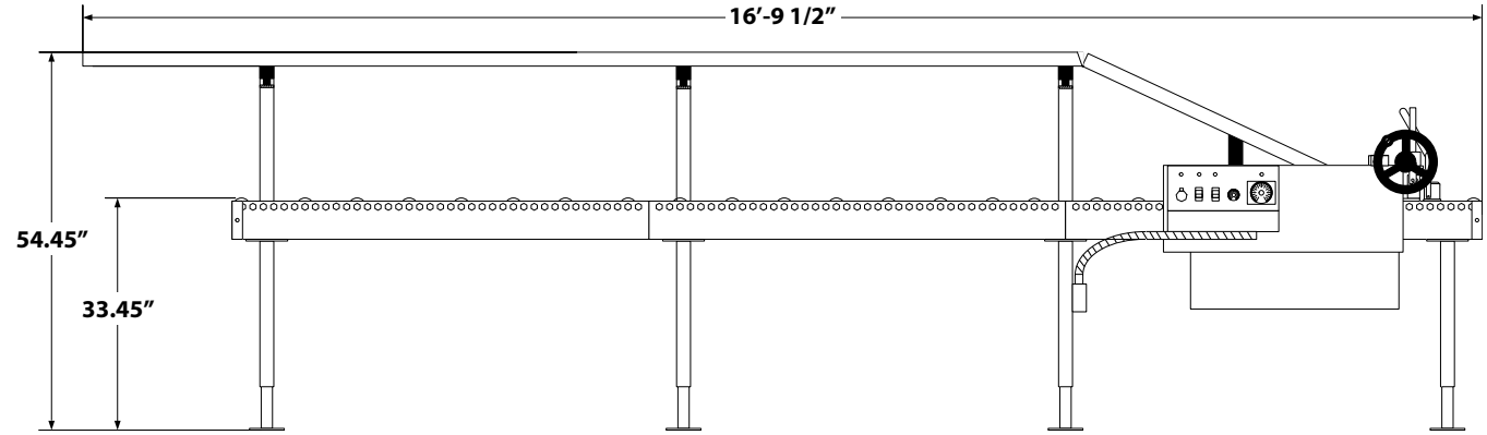
PROFILE VIEW ▶
